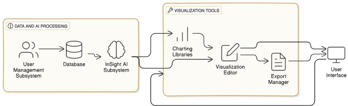
Figure 5.5: Visualization Tools Subsystem Diagram
