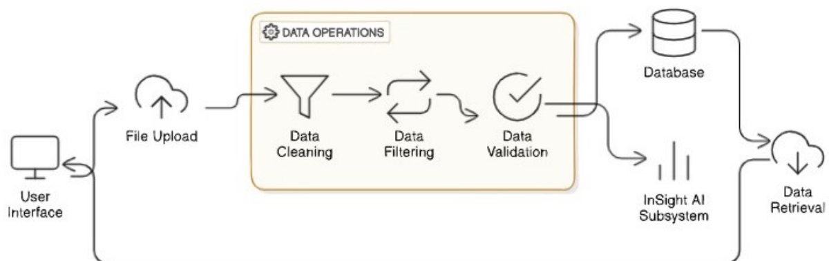
Figure 5.3: Data Handling Subsystem Diagram
