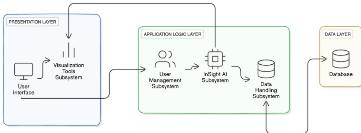
Figure 5.1: High-Level System Architecture Diagram
