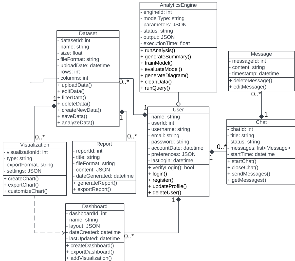
Figure 5.6: UML Class diagram
